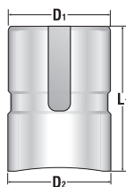
PUNCH DIMENSIONS
